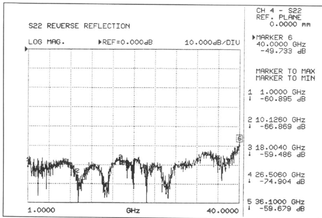
Figure 2: Residual Reflection (Source Match) verified using a Through Line connection after TRL calibration, 1 to 40GHz
