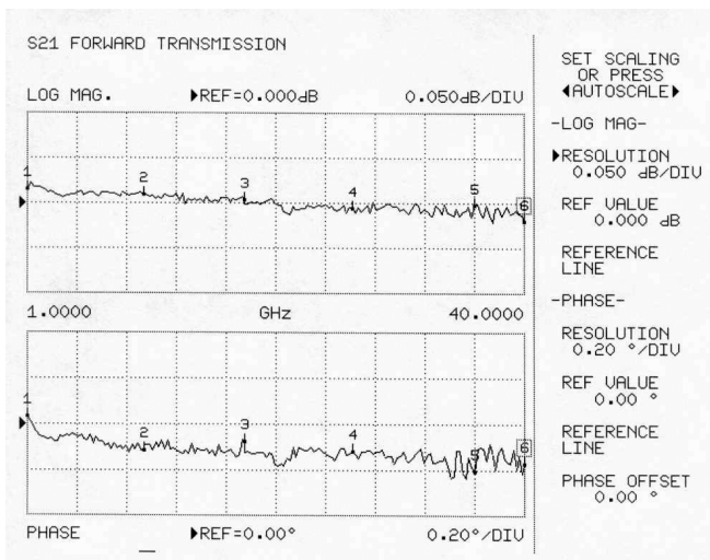
Figure 4: Thru Line Transmission verification (1-40GHz).
