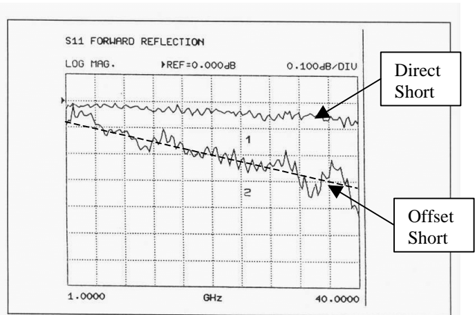
Figure 3: Offset Short Ripple (peak to peak < 0.15dB) 1 to 40GHz
