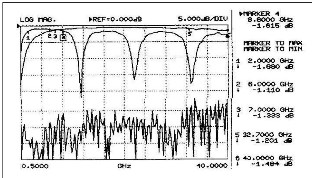
Figure7: Typical CCMT-1808 Min/Max Tuning (the flat response corresponds to a short, high frequency probe, whereas the multiple reflections originate from the wide, low frequency probe)
