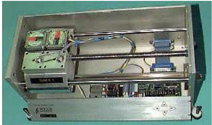
Figure 4: Internal structure of dual axis multioctave tuner (0.7-18 GHz)
