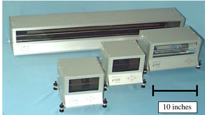
Figure 2 : CCMT models, from the back: 1802-2C (0.2 to 18 GHz), 1808 (0.8 to 18 GHz ), 4006 (6 to 40 GHz) and 4006-2H (fundamental 6 to 40 GHz. harmonic 12-44 GHz)
