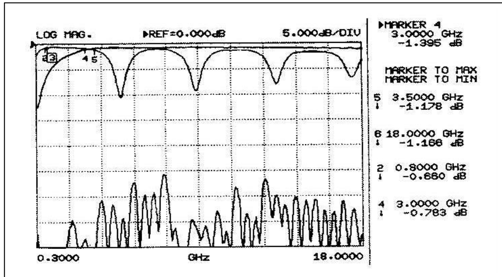
Figure7: Typical CCMT-1808 Min/Max Tuning (the flat response corresponds to a short, high frequency probe, whereas the multiple reflections originate from the wide, low frequency probe)
