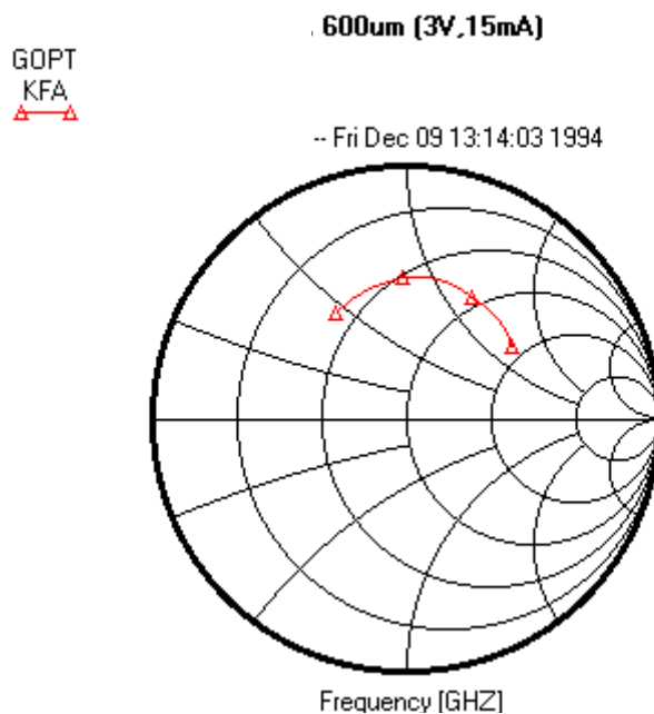
Figure 16: \Gamma_{opt} at 4, 8, 12 & 18 GHz
