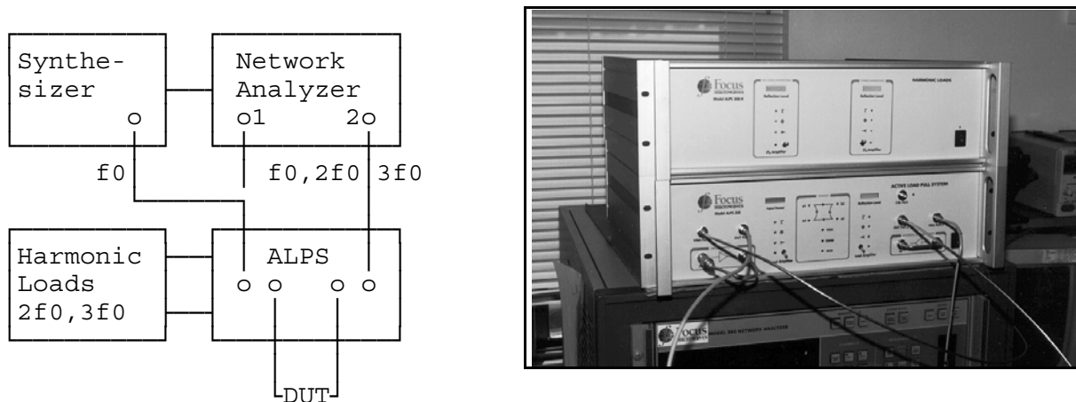
Figure 11: Setup for Load Pull and Harmonic Tuning using ALPS
